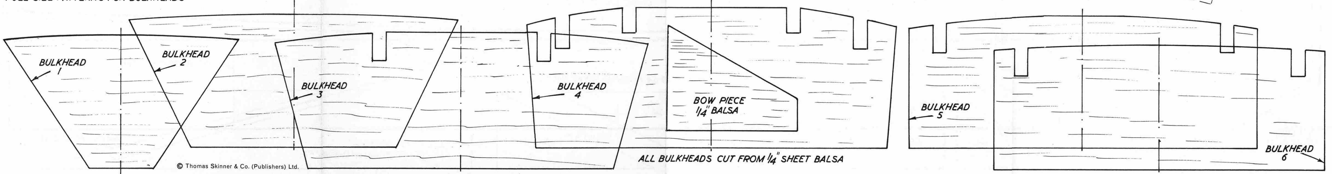
FULL SIZE PATTERNS FOR BULKHEADS
