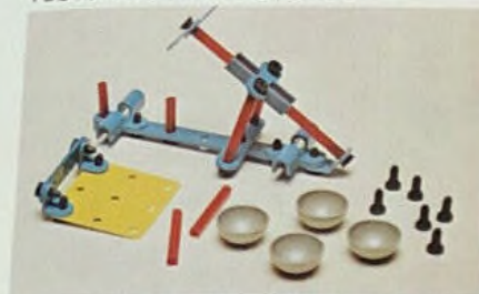
Add Four Domes, Two 2" Tubes To Finish Model
